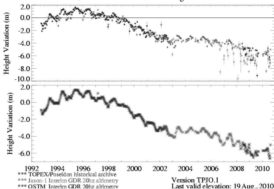
Lake Urmia Height Variations TOPEX 9 Year Geo-referenced 10Hz Along Track Reference
